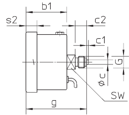
Center back connection, code letters: rm
