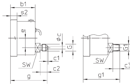
Lower back connection, code letter: r
