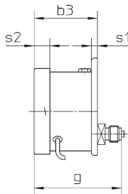
Lower back connection, U-clamp for panel mounting, code letters: rBFr
