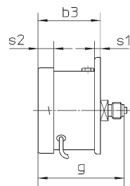
Center back connection, rear mounting flange, code letters: rmRh
